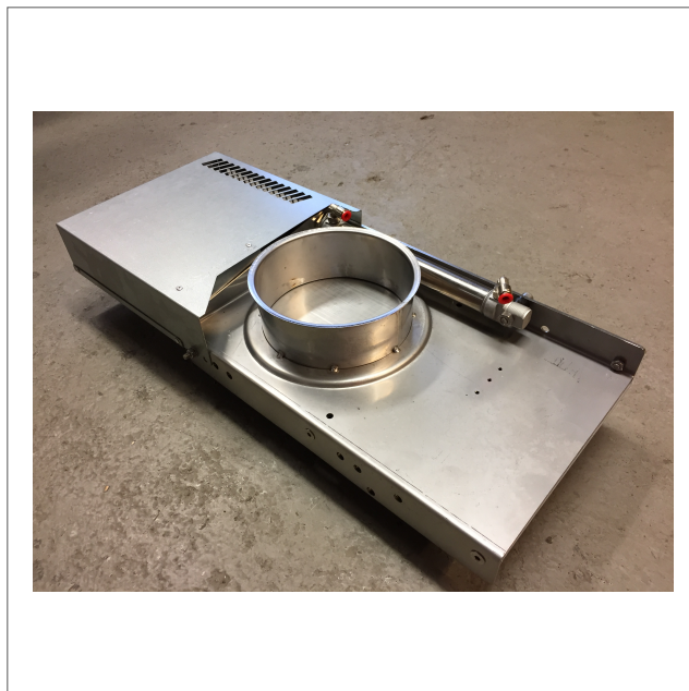
ADCH - cover hood mounted on damper
