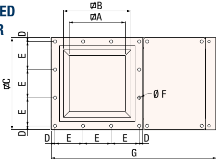
VLR - RECTANGULAR CROSS SECTION
